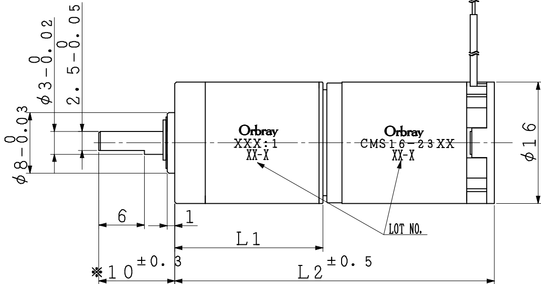
MOTOR LENGTH
